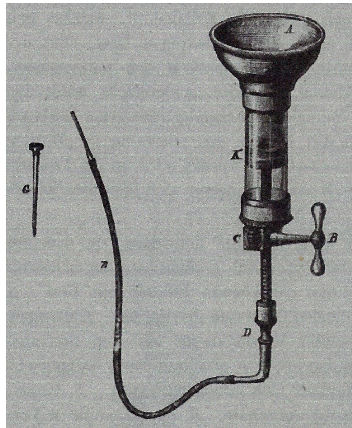
Fig. 11: Mathieu's apparatus
