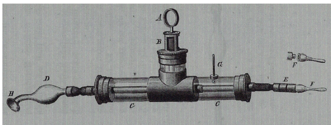
Fig. 5: Mathieu's second apparatus
