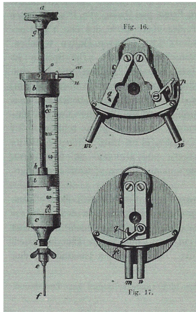
Fig. 15, 16, 17: Mosler's syringe
