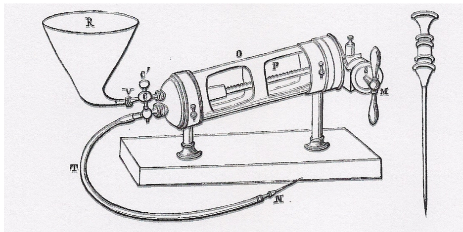
Oré's apparatus #4
